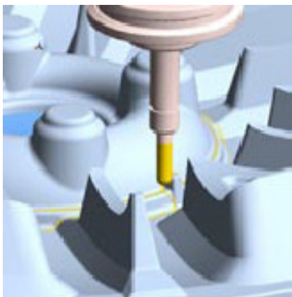
In SolidEdge entworfen, in Edgecam Solid Machinist bearbeitet
